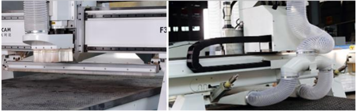
9.0kw ATC spindle with circle tool magazine that could change 12 tools automatically.
